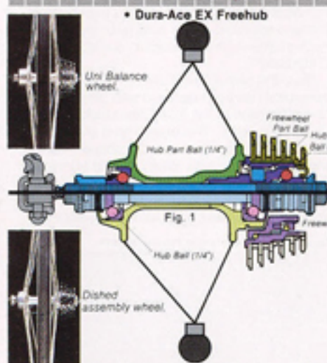
• Conventional Dura-Ace Hub & Freewheel
