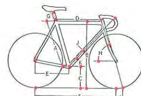
Quantum Series frame Line drawings correspond to chart dimensions.
