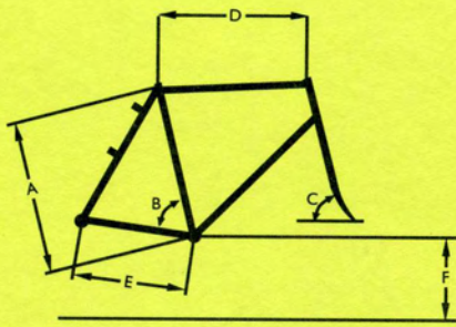
STANDARD MOUNTAIN FRAME GEOMETRY (Inches)
