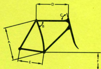
"LITESPEED" ULTIMATE ROAD FRAME GEOMETRY (Centimeters)
