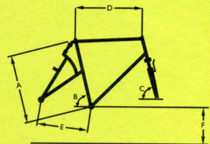
SUSPENDED MOUNTAIN BIKE GEOMETRY (Inches)
